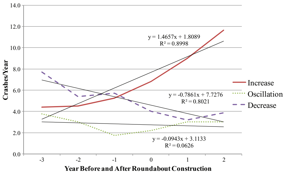
Figure 3. Three temporal trends of roundabout crashes. (Color figure available online).
