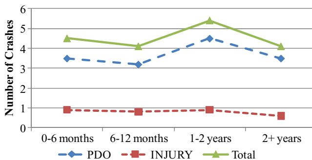
Figure 6. Roundabout crashes postconstruction. PDO = property damage only. (Color figure available online).
