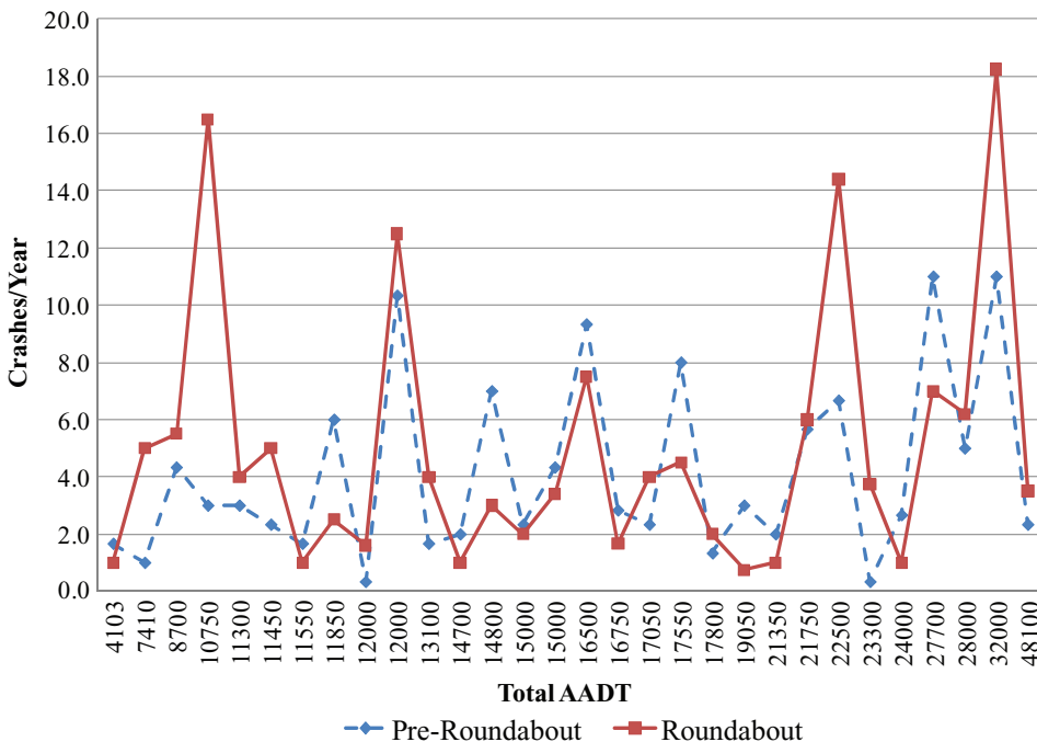
Figure 4. Crashes per year before and after construction of roundabouts. AADT = Average Annual Daily Traffic. (Color figure available online).
