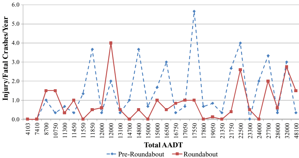
Figure 5. Injury crashes per year before and after construction of roundabouts. AADT = Average Annual Daily Traffic. (Color figure available online).
